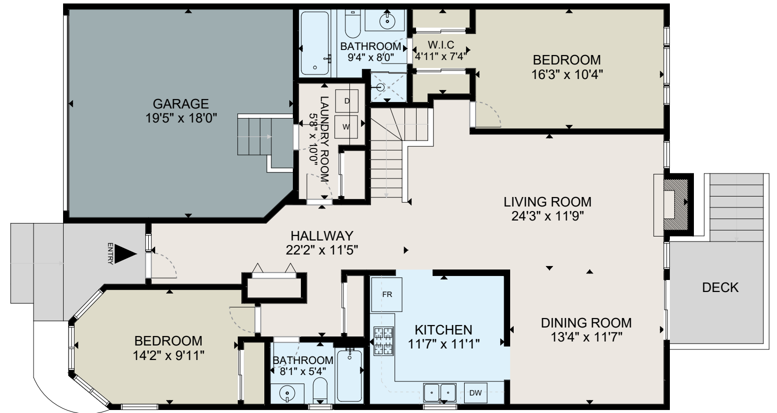
SECOND FLOOR
