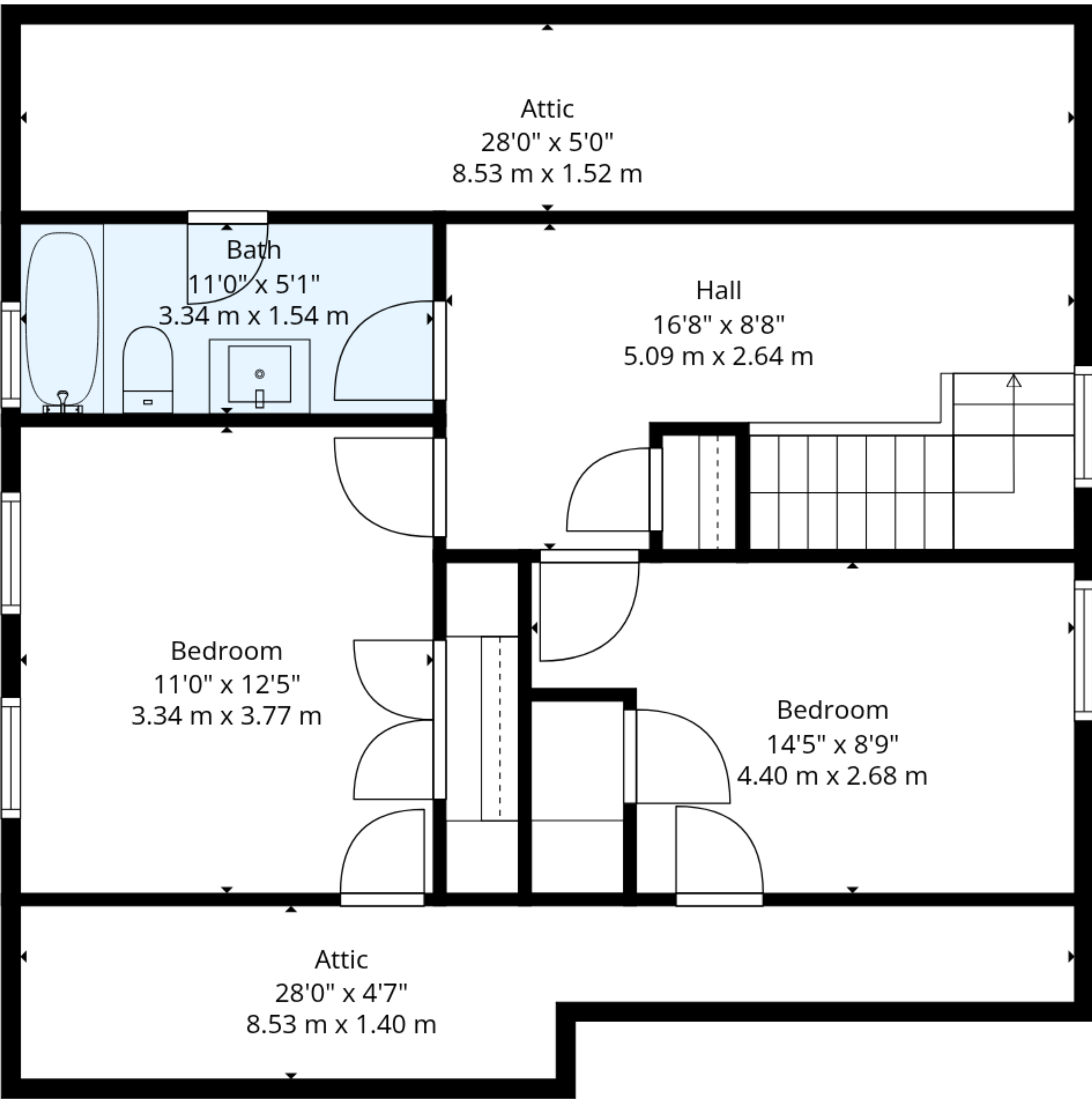
2nd Floor
