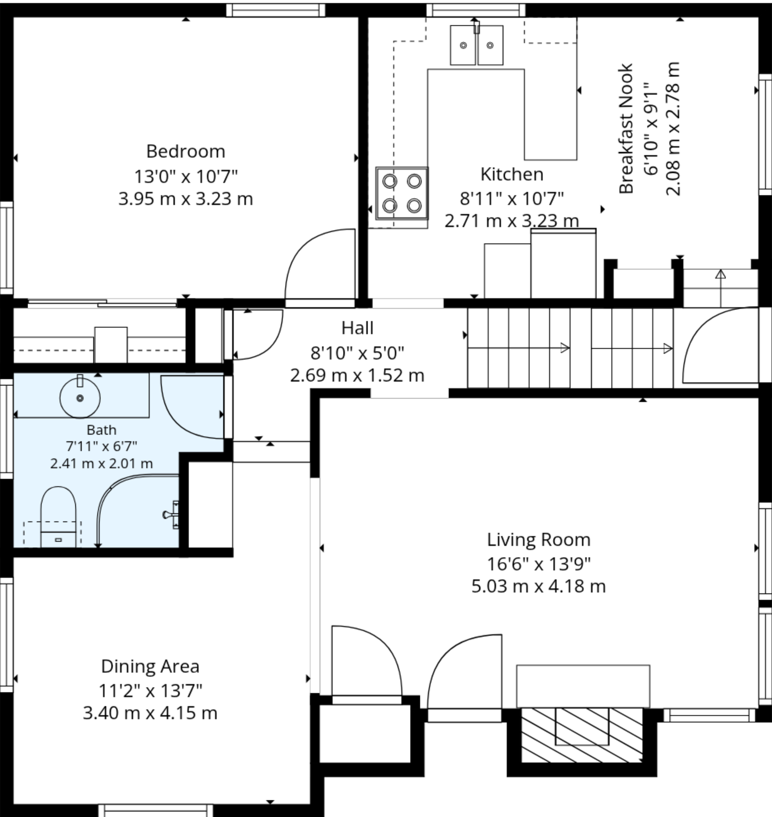
1st Floor
